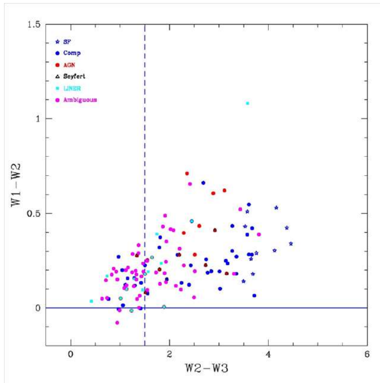
Figure 2. WISE color - color diagram for galaxies with flux error less than 50% and S/N > 15 . The dashed line indicates W2 - W3 = 1.5 . In the graph, galaxies are marked according to the BPT classes.
