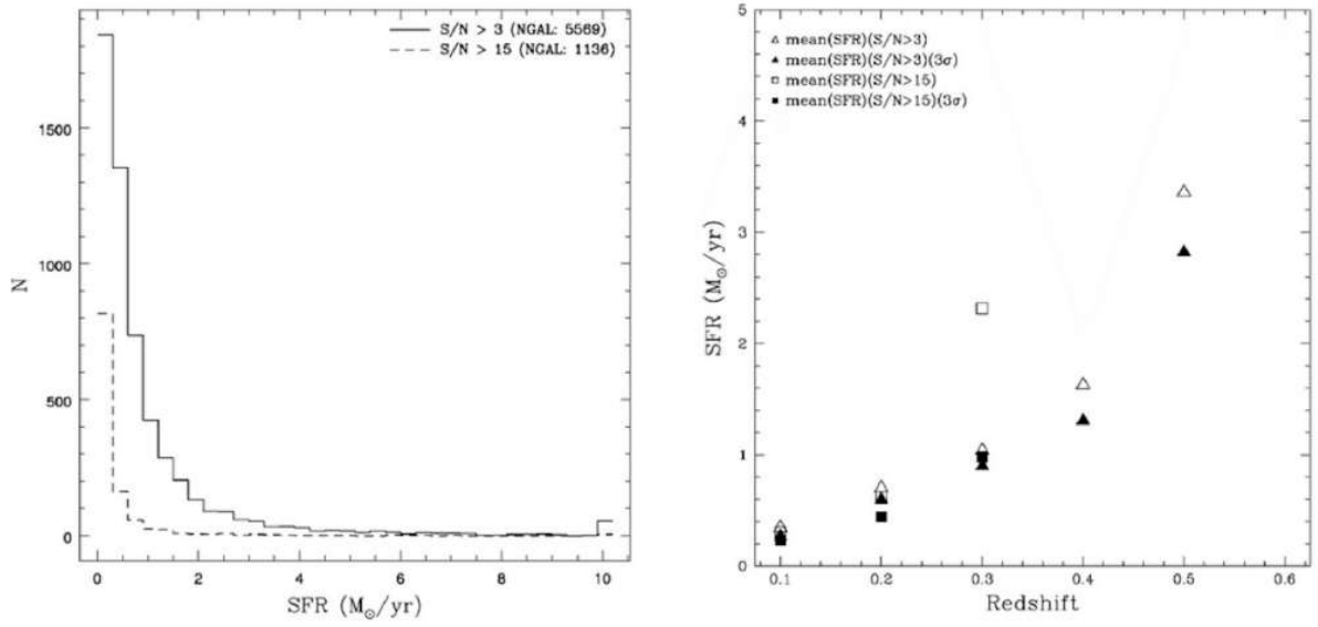
Figure 3. (a) Distribution of calculated SFR values (for SFR < 10 M_{\odot} /year). The solid line indicates galaxies with S/N>3 and the dashed line indicates galaxies with S/N>15. (b) Variation of the mean SFR of the galaxies with redshift for the galaxies with flux error less than 50% and S/N>3 or S/N>15. Empty triangles represent the mean SFR for galaxies with S/N>3 and empty squares are for galaxies with S/N>15. The filled symbols show values when outliers (i.e. 3 \sigma ) are not taken into account.
