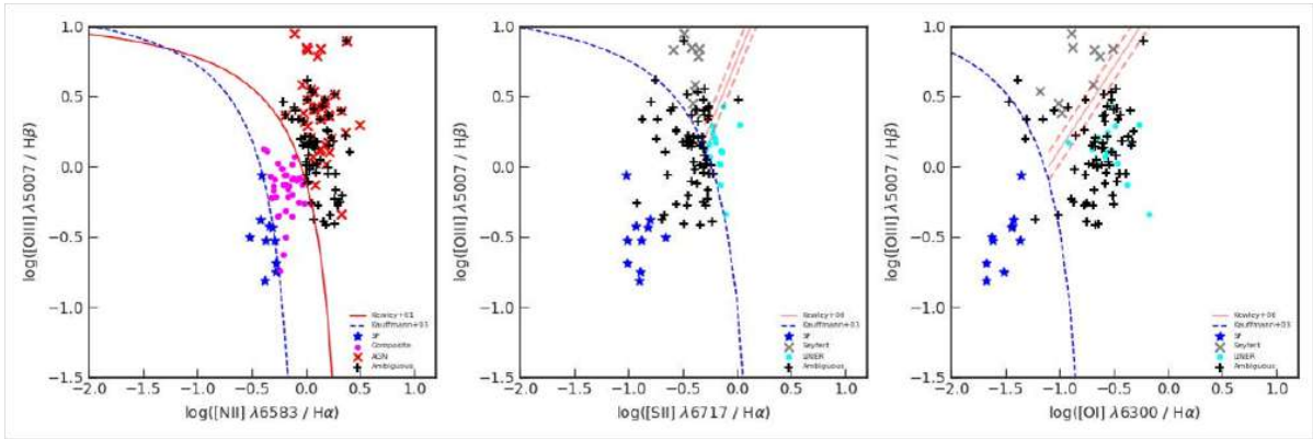
Figure 1. BPT diagram for galaxies with flux error less than 50% and S/N > 15 . The BPT diagrams show star forming galaxies (blue stars - SF), composite galaxies (pink dots - Comp), AGNs (red crosses), Seyfert Galaxies (gray crosses), LINER Galaxies (turquoise crosses), and "ambiguous" galaxies (black pluses).
