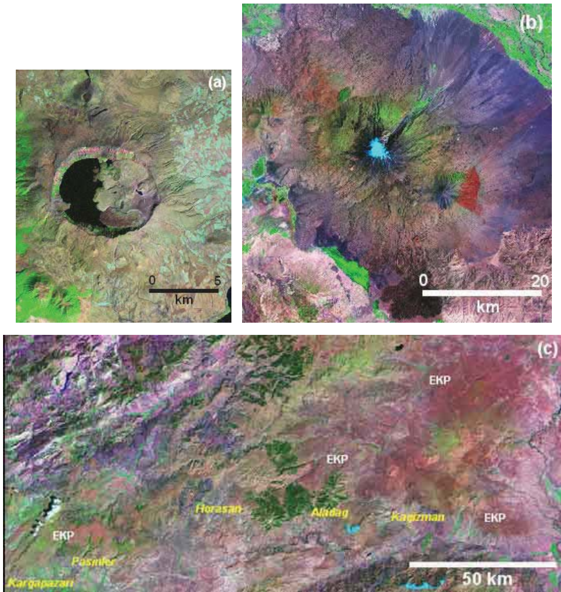
Figure 9. MrSID satellite view of (a) Mt. Nemrut volcano in the south, (b) Mt. Ararat: a double-peaked strato-volcano in the northeast, and (c) the Erzurum-Kars Plateau (EKP) in the northernmost part of the Eastern Anatolia region. On the Erzurum-Kars Plateau (i.e. c) Reddish coloured areas marked EKP correspond to volcanic units, while purple to pinkish areas are either basement units (e.g., areas in the northwest) or young sedimentary cover formations. Vegetation is represented by green areas. For the exact regional locations of Mt. Nemrut and Mt. Ararat, see Fig. 4 .
