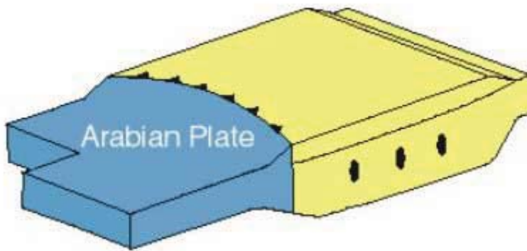
Figure 10: Continental collision and subsequent thickening of the Anatolian crust/lithosphere [Dewey et al., 1986].
