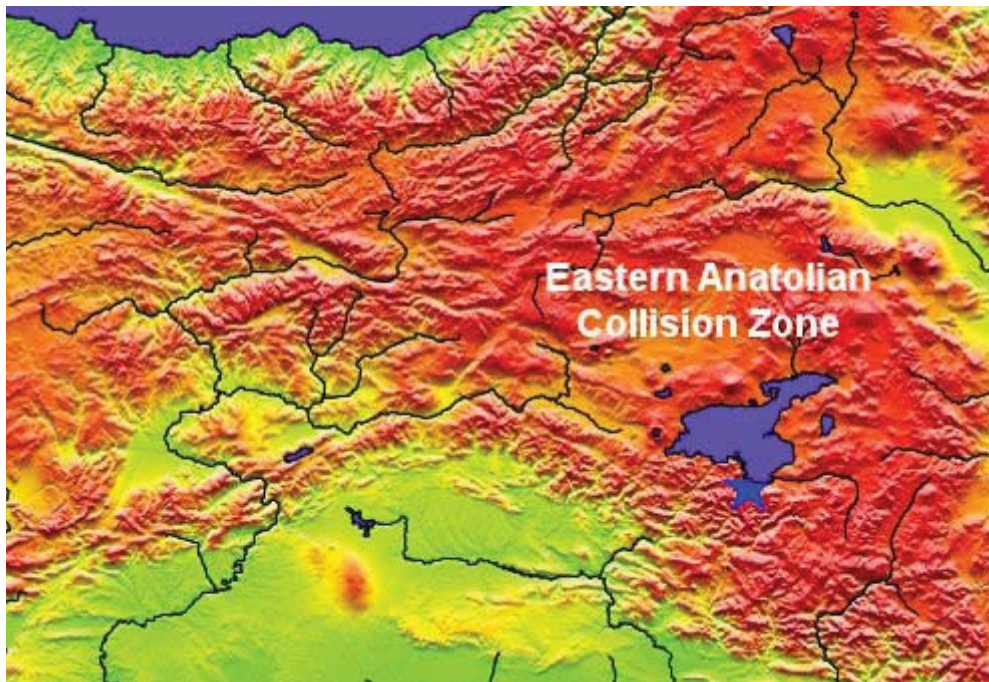
Figure 3. Topographic map showing the Eastern Anatolian plateau with an average elevation of 2 km above sea level. See Figs. 4, 5 and 6 for the main tectonic lines and stratigraphic units.
