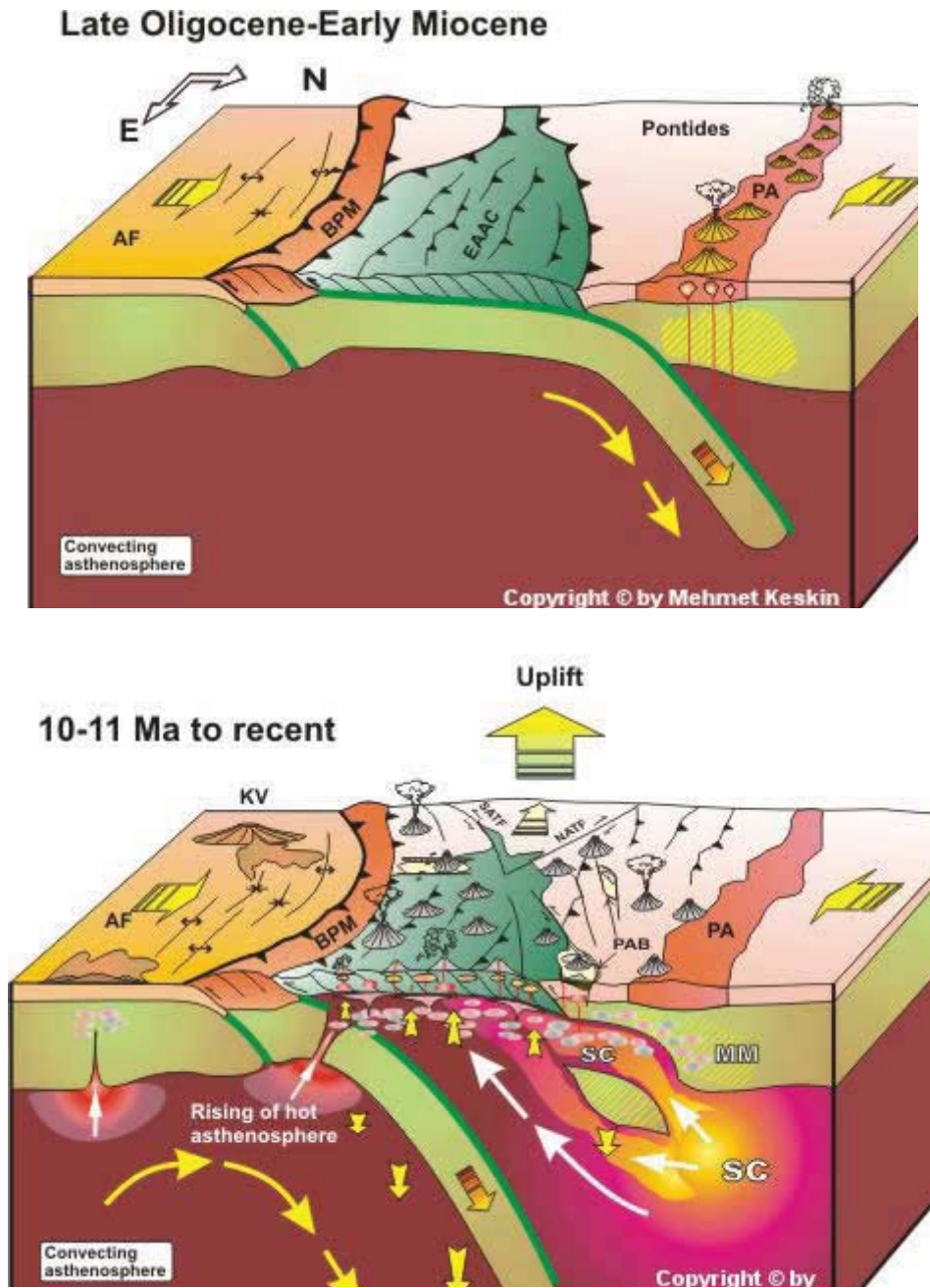
Figure 35. Block diagrams illustrating the slab-steepening & breakoff model for the Eastern Anatolian Collision Zone. Modified from Keskin [2003]. SC: subduction components. White arrows indicate the flow direction of the asthenosphere.
