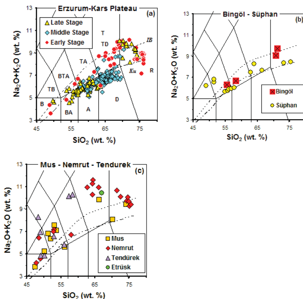
Figure 13. Classification of volcanic units of the Eastern Anatolia region on the total alkali vs silica diagram of Le Bas et al. [1986]. Data for Erzurum-Kars Plateau are from Keskin et al. [1998], the rest are taken from Pearce et al. [1990]. Diagrams are arranged from north to south:
