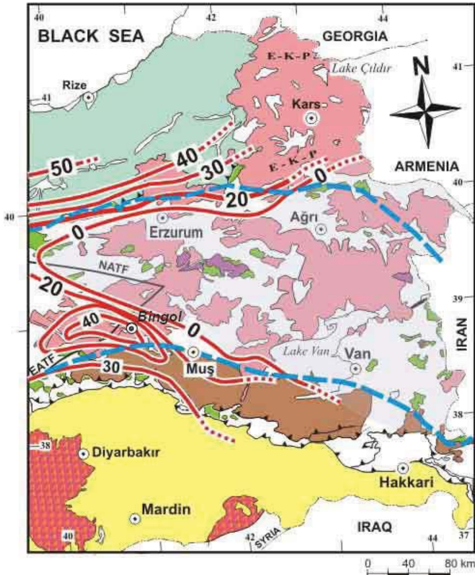
Figure 12. Contours (red) displaying the mantle lid (i.e. lithospheric mantle) thicknesses in km (contours are taken from Fig. 2 of Sengor et al. , 2003). The light bluish-coloured triangular area surrounded by the cities of Agri, Erzurum, Bingol and Van in the centre of the figure represents the area with no mantle lid. Thick, dotted dark-blue lines represent the northern and southern borders of the Eastern Anatolian Accretionary Complex (also see Fig. 5). Note that areas of inferred complete lithospheric detachment almost exactly coincide with the extent of the Eastern Anatolian Accretionary Complex (i.e. the EAAC).
