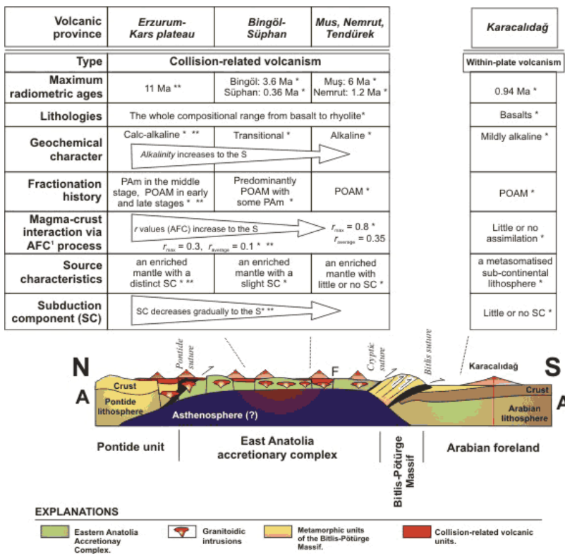
Figure 8. Cross section summarizing the crustal structure and petrologic/geochemical properties of the collision-related volcanic units across the Eastern Anatolia Region [Keskin, 2003]. The crustal and lithospheric thicknesses are from Sengor et al. [2003] and Zor et al. [2003]. The direction of the cross section (A-A') is shown in Fig. 4. Source of geochemical data: *Ercan et al. [1990], **Pearce et al. [1990], ***Keskin et al. [1998]. SC: subduction component, AFC: Assimilation combined with fractional crystallization process, r : ratio of the rates of mass assimilation and mass crystallization. F: strike-slip faults.
