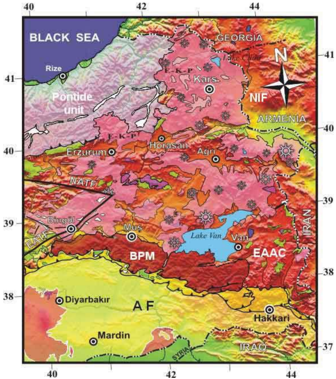
Figure 6. Topographic map of the Eastern Anatolia Collision Zone (EACZ) over which the main tectonic units as well as collision-related volcanics are superimposed. NIF: Northwest Iranian Fragment, BPM: Bitlis-Poturge massif, EAAC: Eastern Anatolian Accretionary Complex, AF: Arabian Foreland. For more explanation, see Figs. 4 and 5 .
