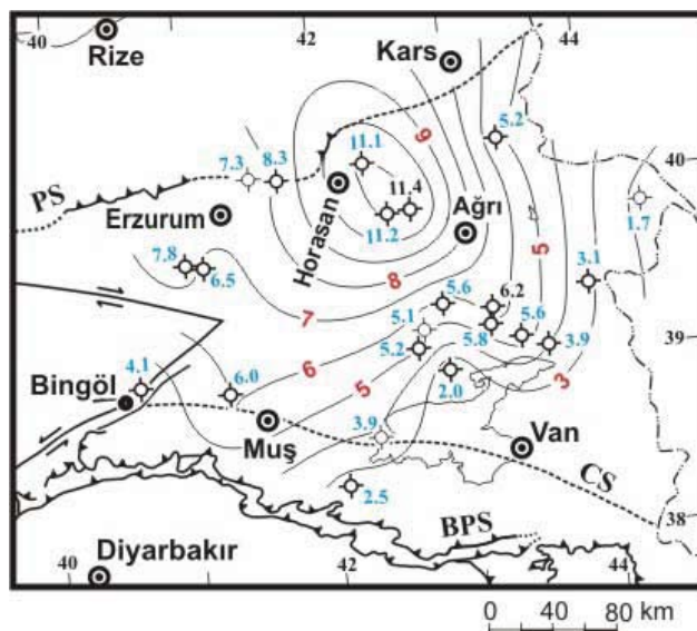
Figure 7. Distribution of the oldest radiometric ages of the volcanic units. Ages are from Pearce et al. [1990], Ercan et al. [1990] and Keskin et al. [1998]. Initiation ages of the volcanism are contoured in 1-Myr intervals. PS: Pontide suture, BPS: Bitlis-Poturge suture, CS: inferred cryptic suture between the EAAC and BPS. Figure from Keskin [2003].
