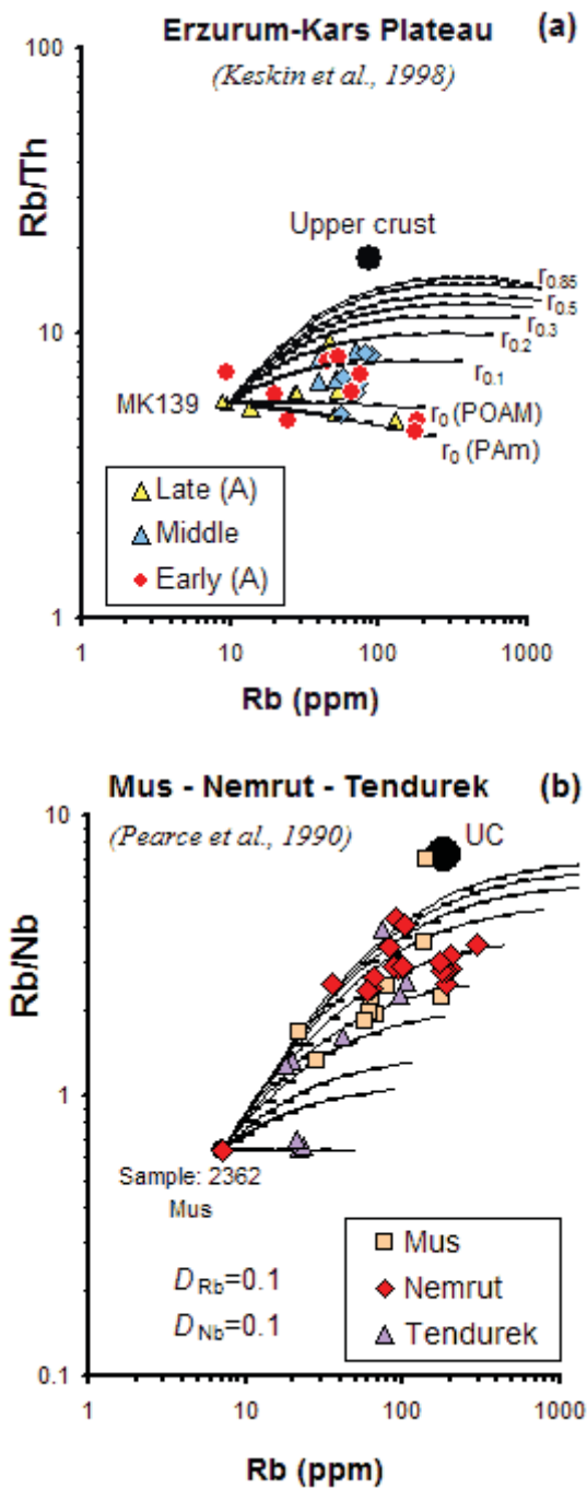
Figure 18. Diagrams showing the results of assimilation-fractional crystallisation (AFC) modelling. The modelling was conducted using the AFC equations of De Paolo [1981]. Bulk partition coefficients are inset in the diagrams. Parental magma compositions correspond to the basaltic sample MK139 (Erzurum-Kars Plateau; Keskin et al., 1998) and sample 2362 (Mus-Nemrut-Tendurek; Pearce et al., 1990), and the average crustal composition of Taylor & McLennan [1985].
