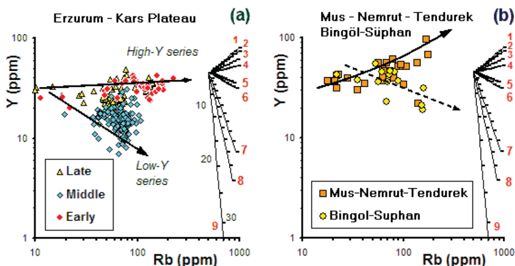
Figure 17. Rb vs. Y diagram displaying theoretical Rayleigh fractionation vectors for 50% crystallisation of the phase combinations (given below) from a common magma composition. Tick marks on each vector correspond to 5% crystallisation intervals. The data for the Erzurum-Kars Plateau are from Keskin et al. [1998], while those from the Mus-Nemrut-Tendurek and Bingöl-Süphan volcanoes in the south are from Pearce et al. [1990]. Bulk partition coefficient values used in the modelling are those given in Table 2 of Keskin et al. [1998]. The FC vectors have been modelled using the “FC-Modeler program” of Keskin [2002].
