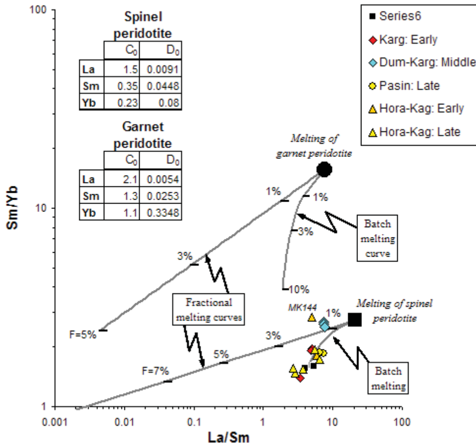
Figure 19. La/Sm vs. Sm/Yb plot showing theoretical melting curves plotted along with the basic samples ( SiO_2 < 57\% ) from the Erzurum-Kars Plateau. Fractional and batch melting equations of Shaw [1970] were used to construct the melting model. F : weight fraction of melt produced.
