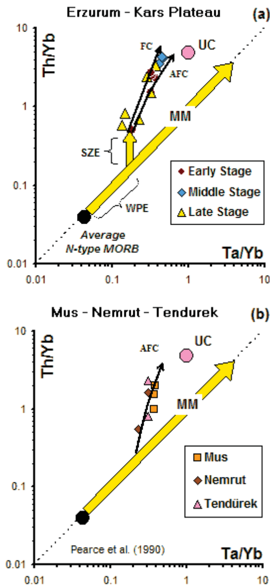
Figure 16. Th/Yb vs. Ta/Yb diagram [after Pearce, 1983] for basic and intermediate lavas ( \text{SiO}_2 < 60\% ) from the Eastern Anatolia Collision Zone. Data from the Mus-Nemrut-Tendurek volcanoes are from Pearce et al. [1990]. MM: mantle metasomatism array; SZE: subduction zone enrichment; WPE: within-plate enrichment; UC: upper crustal composition of Taylor & McLennan [1985]; FC: fractional crystallisation vector; AFC: assimilation combined with fractional crystallisation curve. The FC curve has been modelled for 50% crystallisation of an assemblage consisting of 50% plagioclase and 50% amphibole from a basic magma. The AFC vector has been drawn for an "r" value of 0.3. Note that lavas of the Erzurum-Kars Plateau contain a distinct subduction zone enrichment (SZE) signature.
