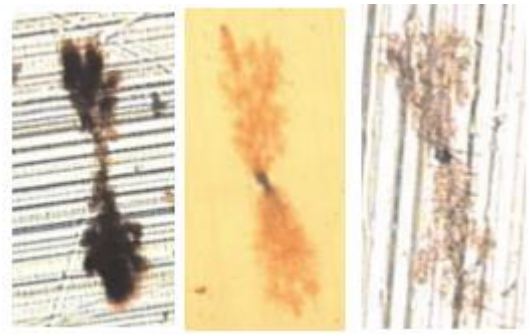
Fig. 3. Bow-tie water tree [14]
