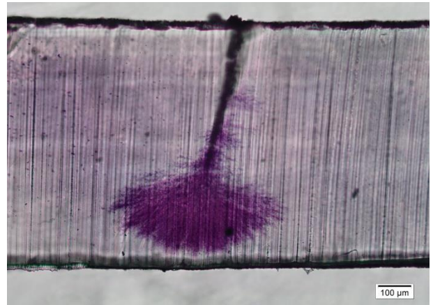
Fig. 16. Microscope image of vented type water tree (1M, 24 kV PP , 3 kHz, 24 hours, 84.2 mS/cm )
