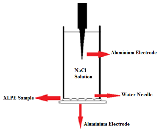
Fig. 4. Water treeing test setup
