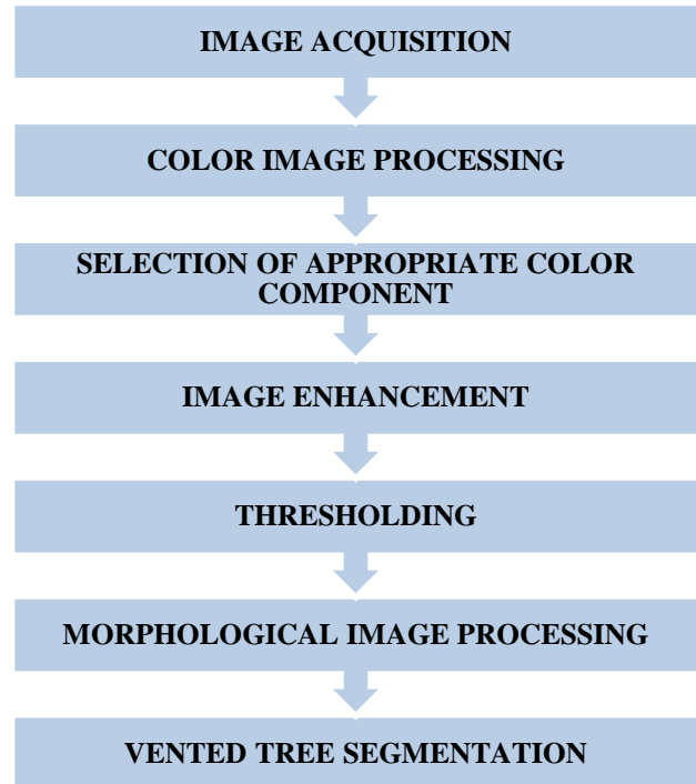
Fig. 6. The steps of segmentation of vented water trees.
