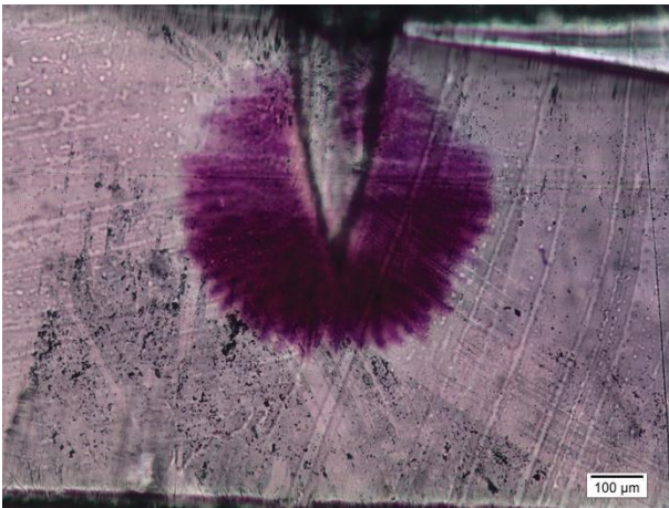
Fig. 12. Microscope image of vented type water tree (1M, 24 kV PP , 3 kHz, 24 hours, 84.2 mS/cm )
