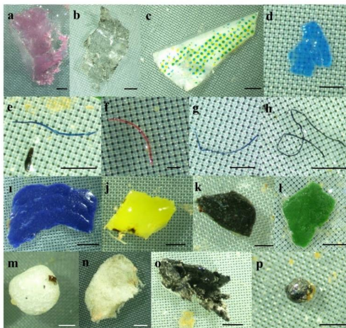
Figure 5. Examples of films (a-d), fibres (e-h), fragments (i-l), foams (m-o), microbead (p) collected from surface waters (scale bar=500 \mu m)
