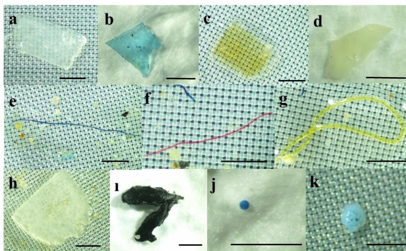
Figure 9. Examples of films (a-d), fibres (e-g), fragments (h-i), and microbeads (j-k) collected from surface waters (scale bar=500 \mu m)
